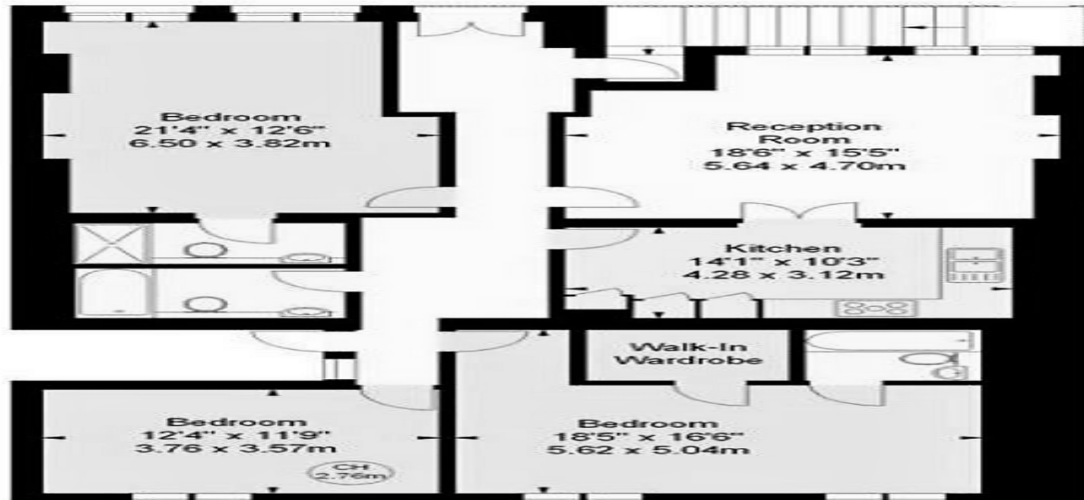
First Floor
